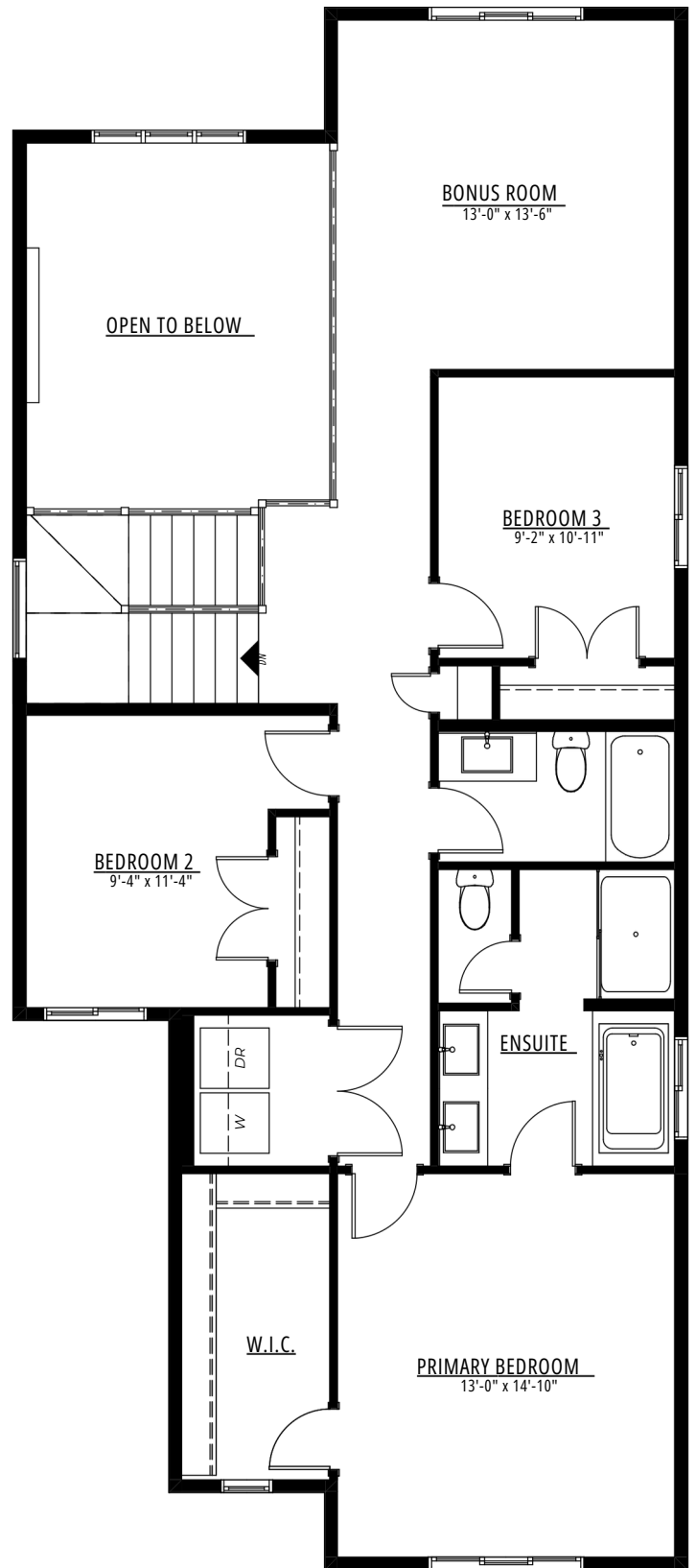
SECOND FLOOR
